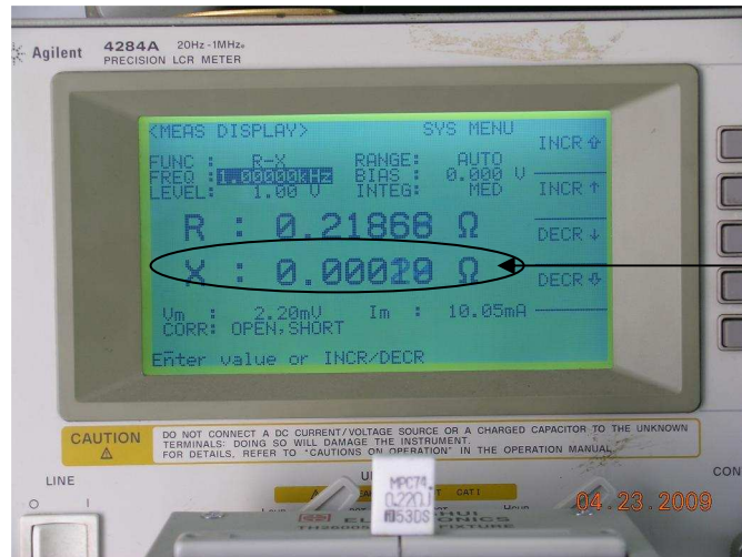
Measurement setup
