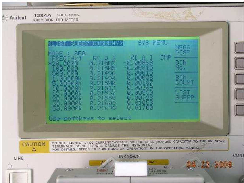
Sweep result for a cheap wire wound resistor
